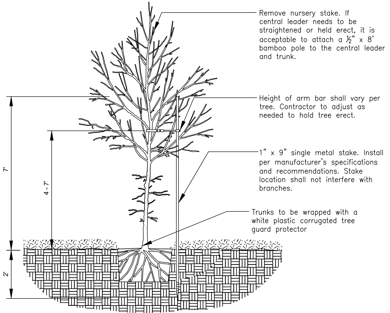
SECTION VIEW
